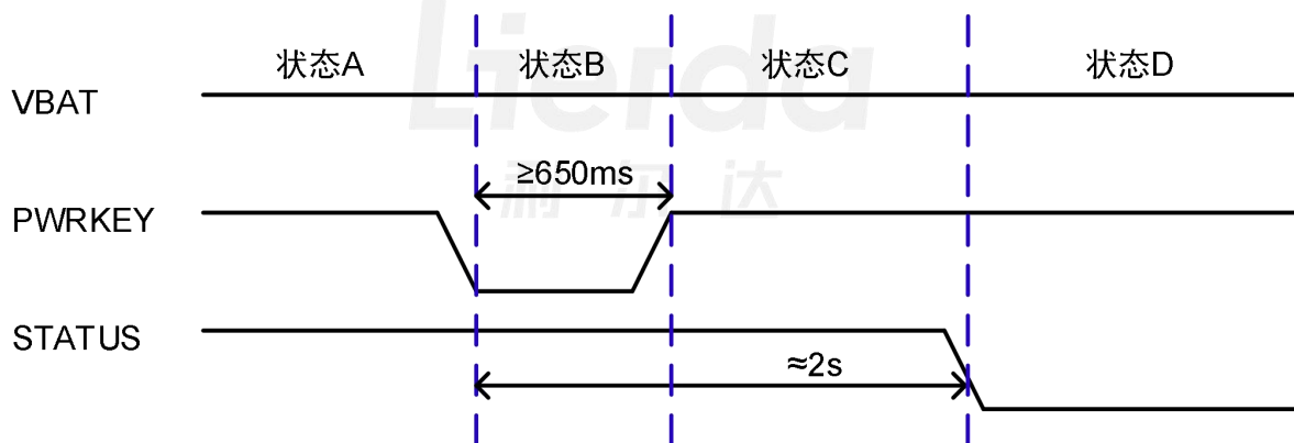
Figure 3-7 Power Key Shutdown Timing Diagram
