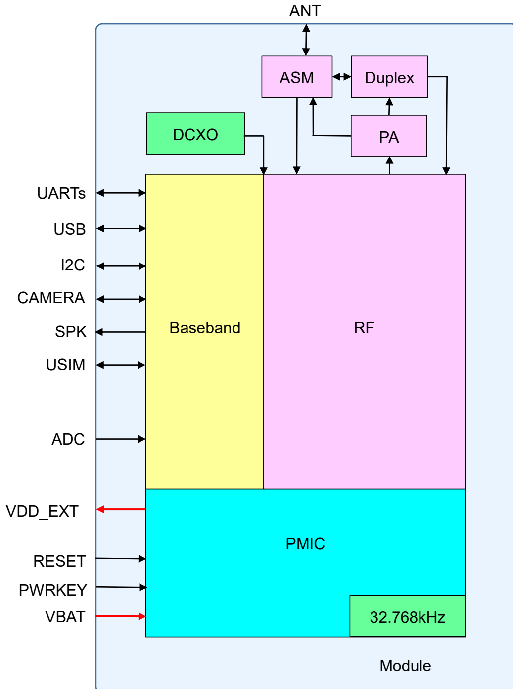
Figure 2-1 Module Functional Block Diagram
