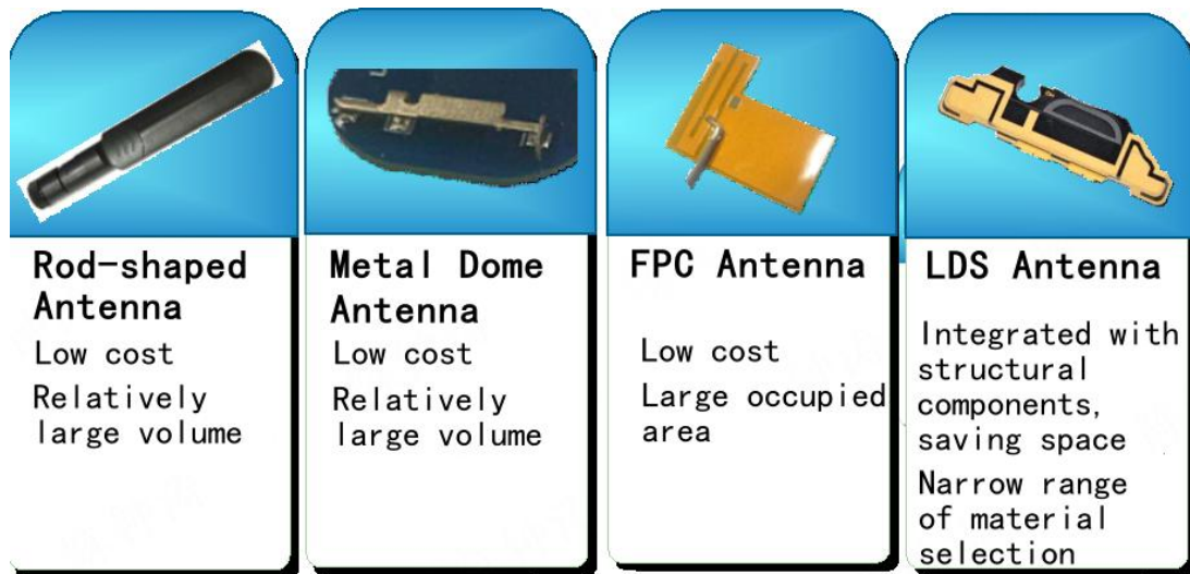
Figure 5-4 Common Antenna Types for CAT1
