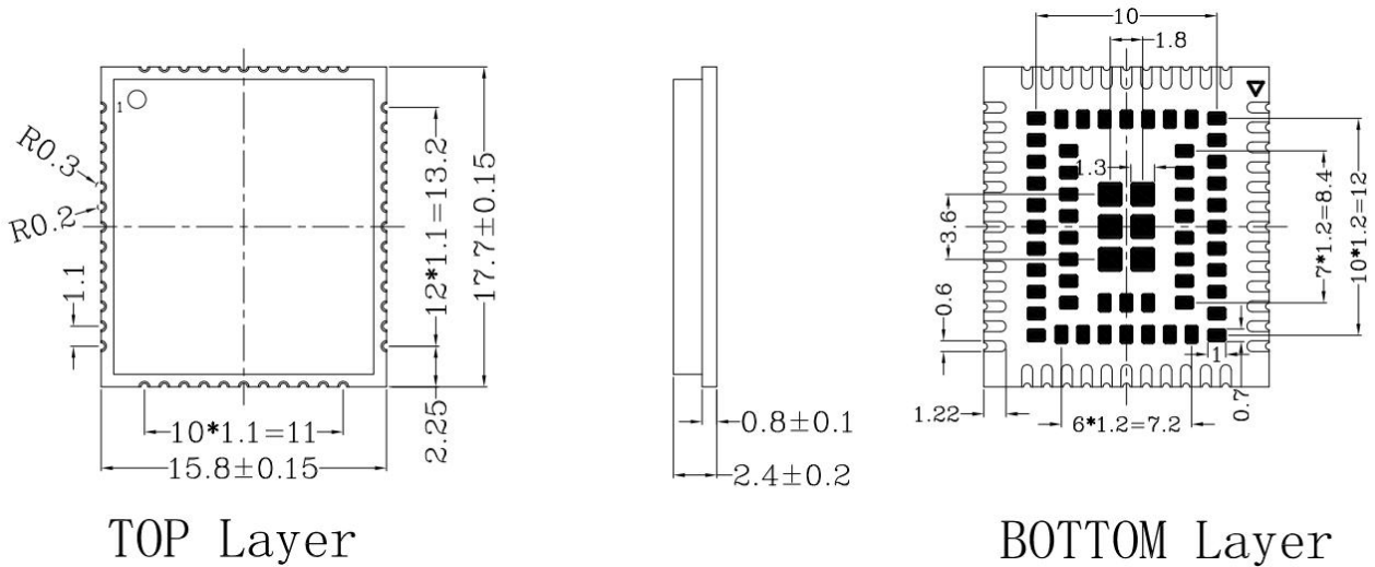
Figure 7-1 Module Mechanical Dimension Drawing (unit: mm)
