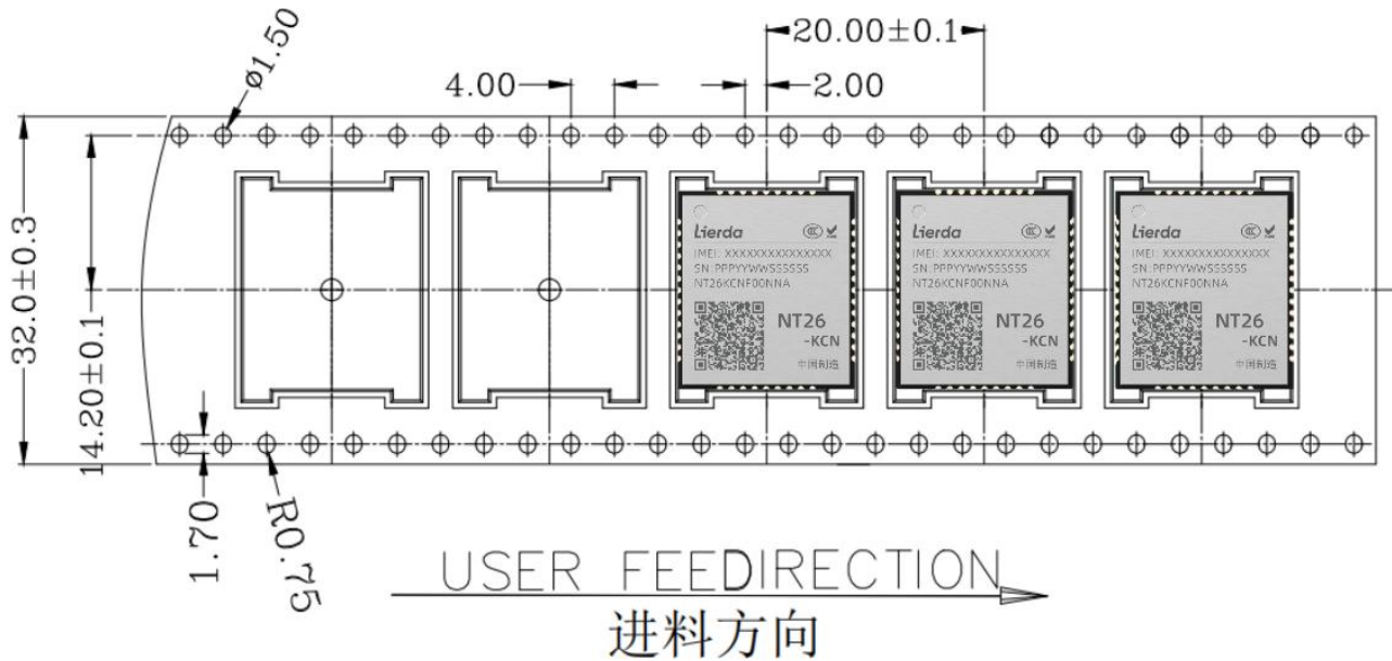
Figure 8-3 Loading Direction Indicator Diagram
