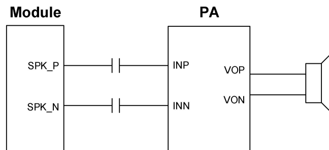
Figure 4-8 SPK Application Reference Circuit
