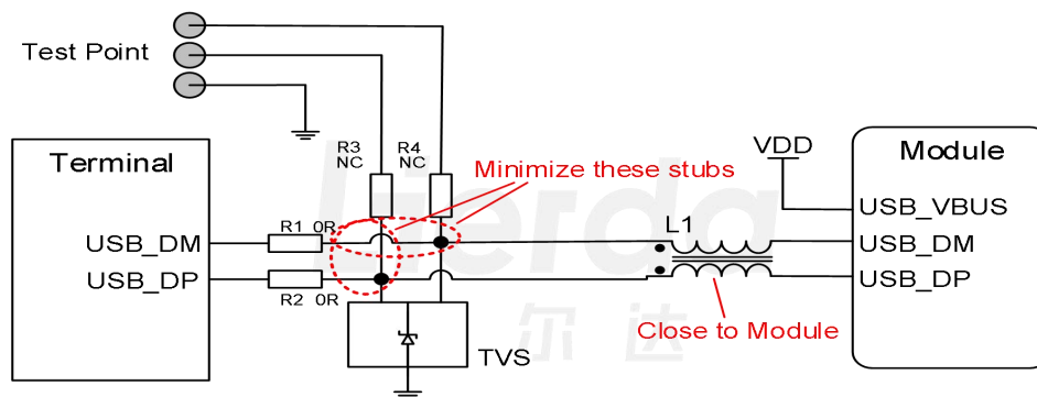
Figure 4-2 USB connected MCU reference design
